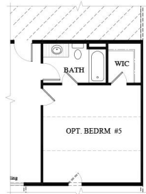
OPTIONAL BED & BATH ILO LOFT
